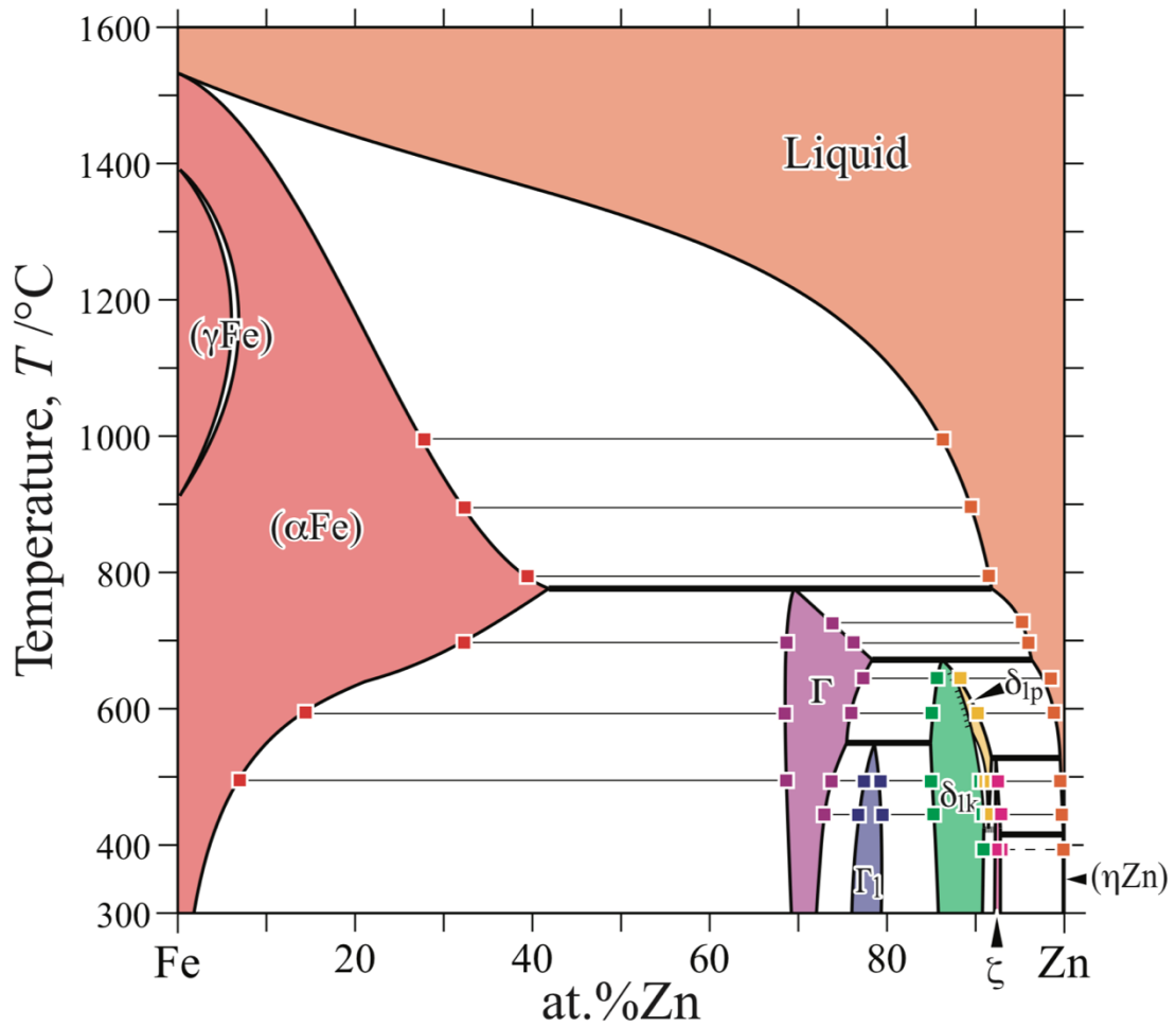
FIG. 1 Phase equilibria of the Zn-Fe binary system experimentally determined by alloying method.
